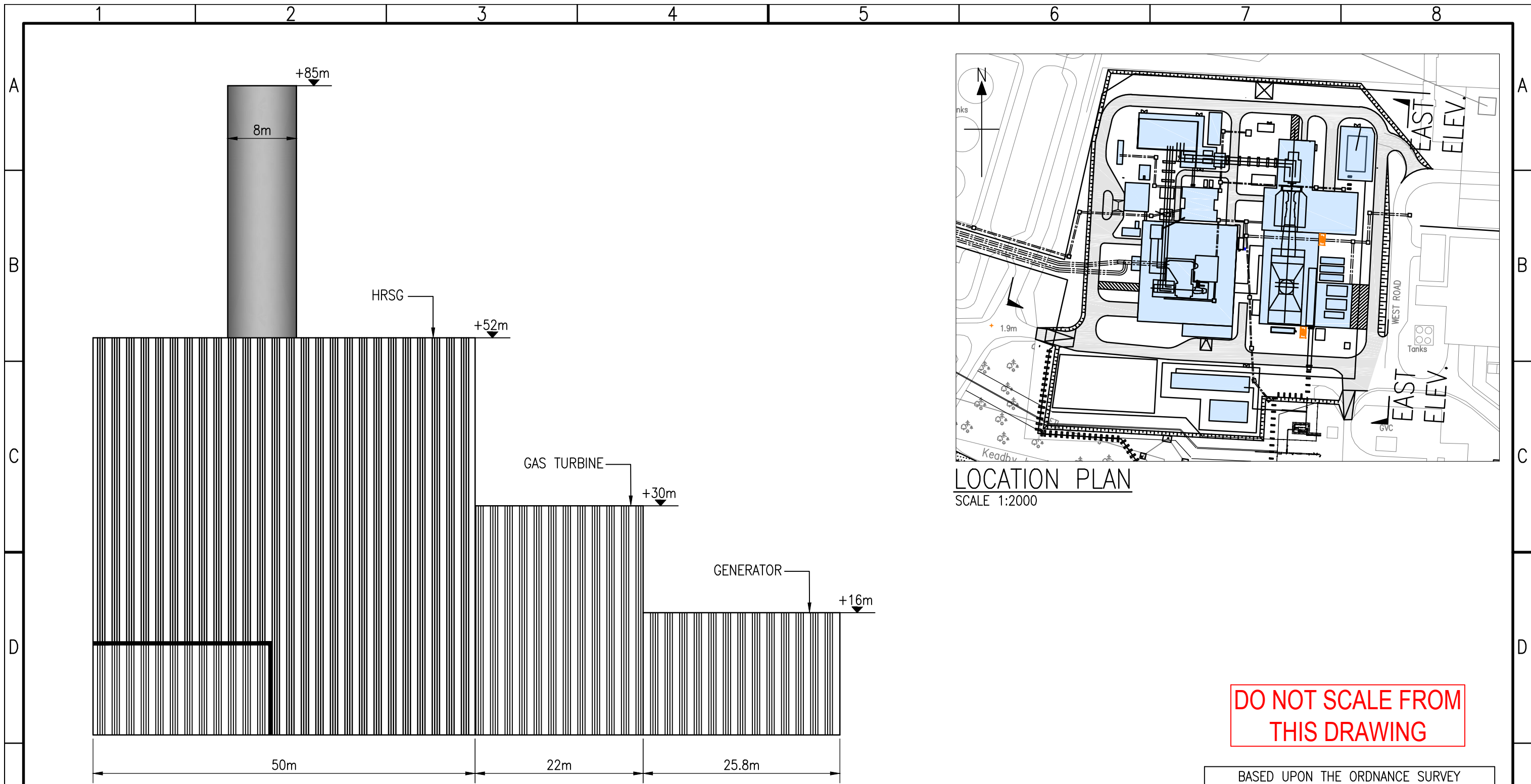
EAST ELEVATION SCALE 1:500
